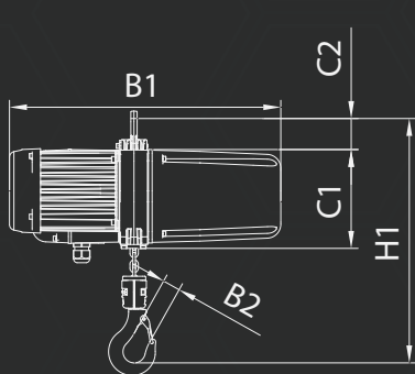
Eyebolt Suspension
