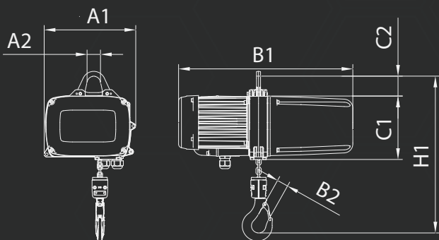
Eyebolt Suspension
