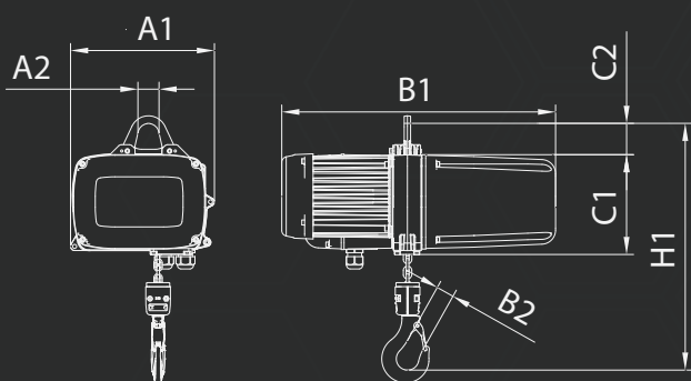
Eyebolt Suspension
