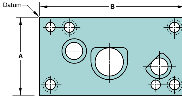
View from the punch head side.
