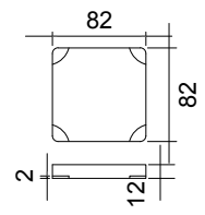
DRAIN COVER
