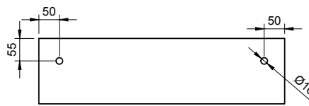
REAR VIEW
