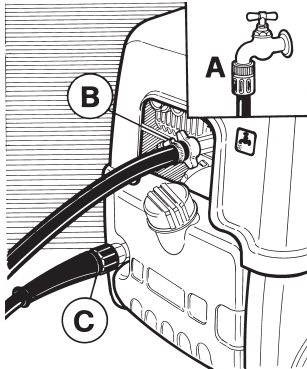
Water circuit connection.
