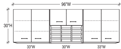
WALL MODULE: 84514 E96 WC (no locks) 84514 F96 WC (with locks)
