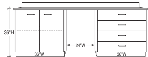
BASE MODULE: 84514 E96 BC (no locks) 84514 F96 BC (with locks)
