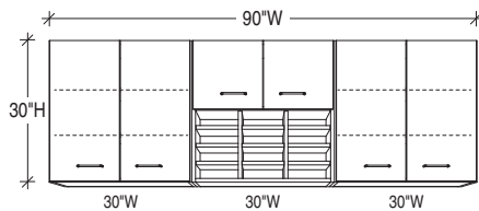
WALL MODULE: 84514 E90 WC (no locks) 84514 F90 WC (with locks)
