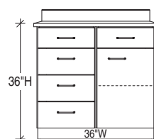
BASE MODULE: 84504 E36 BC (no locks) 84504 F36 BC (with locks)
