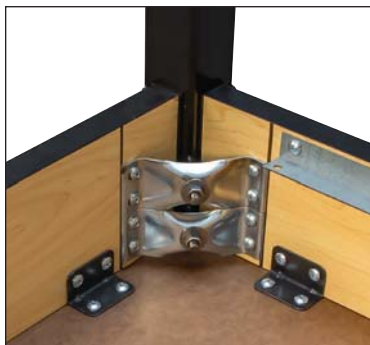
1" apron rails with double gusset leg brackets
