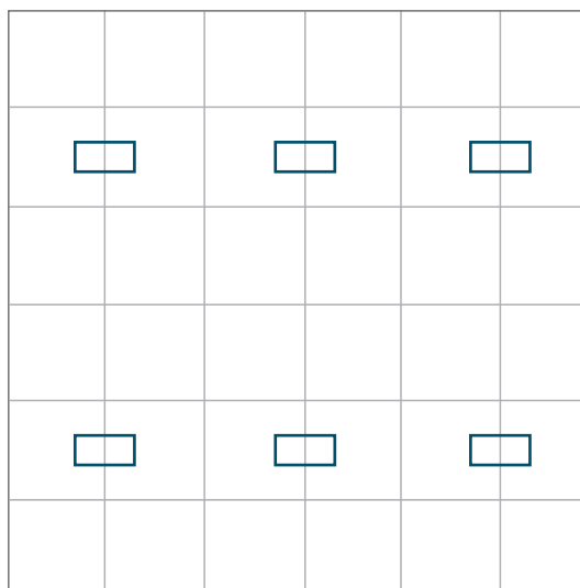
6 × Garage Lights 353 lx avg. @ 0.8m working plane
