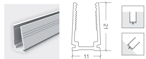
PLASTIC PROFILE
