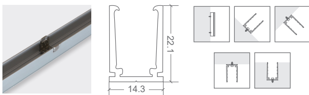
SELF-LOCKING ALUMINIUM PROFILE / MOUNTING CLIP
