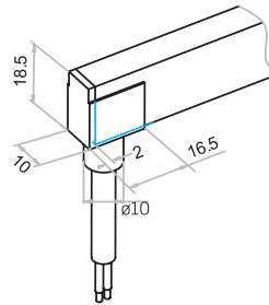
FLEXIBLE CONNECTOR
