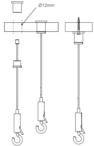
Pendant Coupler WHITE BL-CS-PCW BLACK BL-CS-PCB For use over track joins
