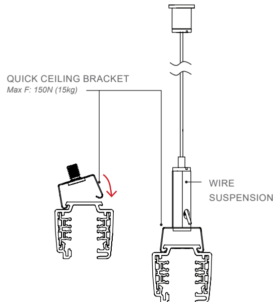
Quick Ceiling Bracket WHITE BL-CS-QCBW BLACK BL-CS-QCBB
