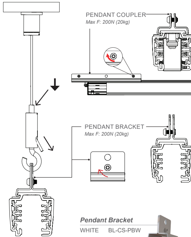
Pendant Coupler WHITE BL-CS-PCW BLACK BL-CS-PCB For use over track joins
