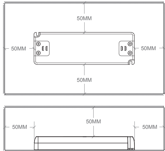
Maintain 50mm space around sides of power supply
