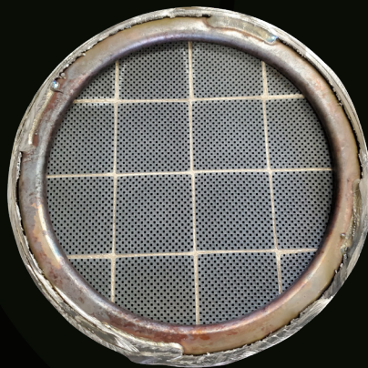
UNITIZED DPF
