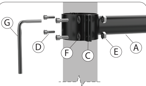
2A. Align both sides of the hoop (A and C) to the chair's cylinder.
