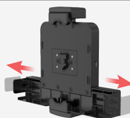
ADJUSTABLE HOLDER FOR DIFFERENT SIZES
