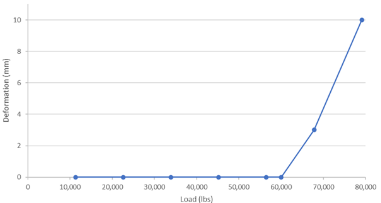
Deflection Plastic Trench Support
