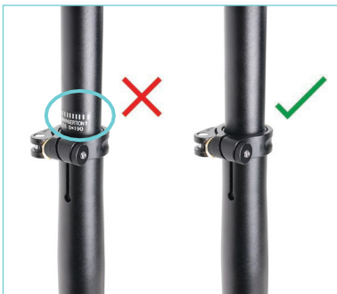
Handlebar Stem
