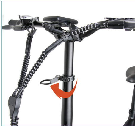
Step 7: Adjust handlebar height and lock it.
