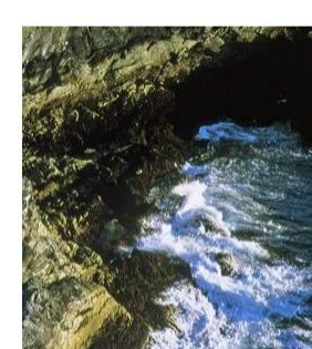
Tidal Forces
