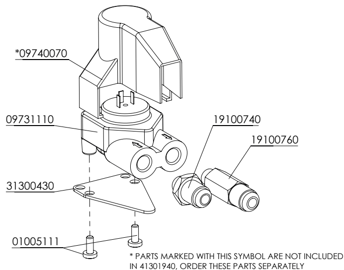
41301940 - FLOWMETER ASSEMBLY BARISTA T D.8
