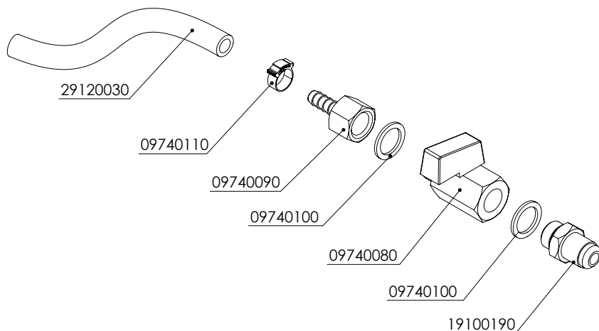
41300160 - DRAIN TAP BARISTA T ASSY.
