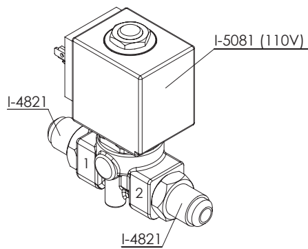
PM-541 - HOT WATER ELECTROVALVE ASSY BABY T 110V
