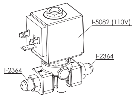
PM-660 - FILLING ELECTROVALVE ASSEMBLY BABY T PLUS ETL 110V
