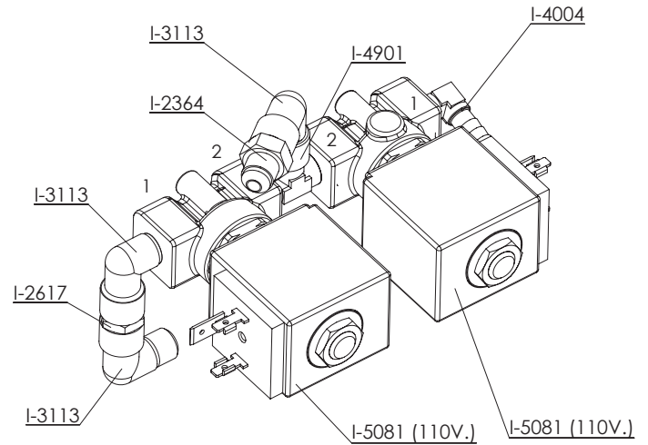
PM-645 - INPUT SELECTOR ASSEMBLY BABY T PLUS ETL 110V
