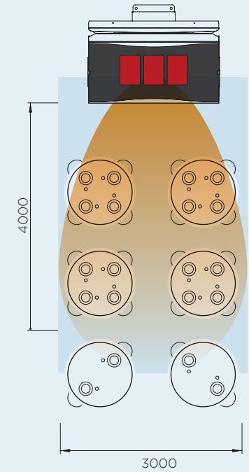
HEATING APPROXIMATELY 15M 2 25MJ HEATING POWER
