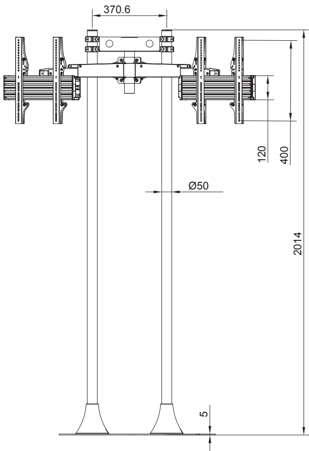
Technical measurements(mm)
