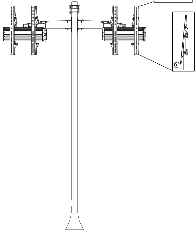
Technical measurements(mm)
