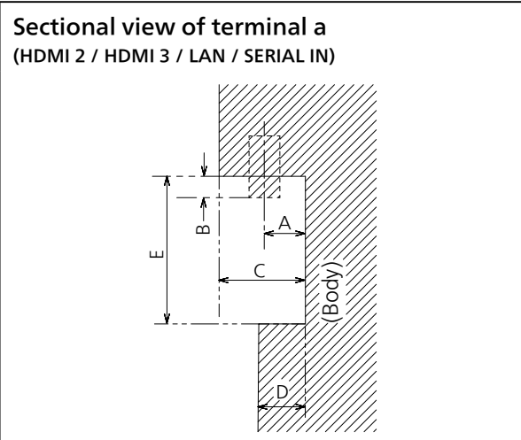
Terminal a 43CQ2U Terminal (Bottom)
