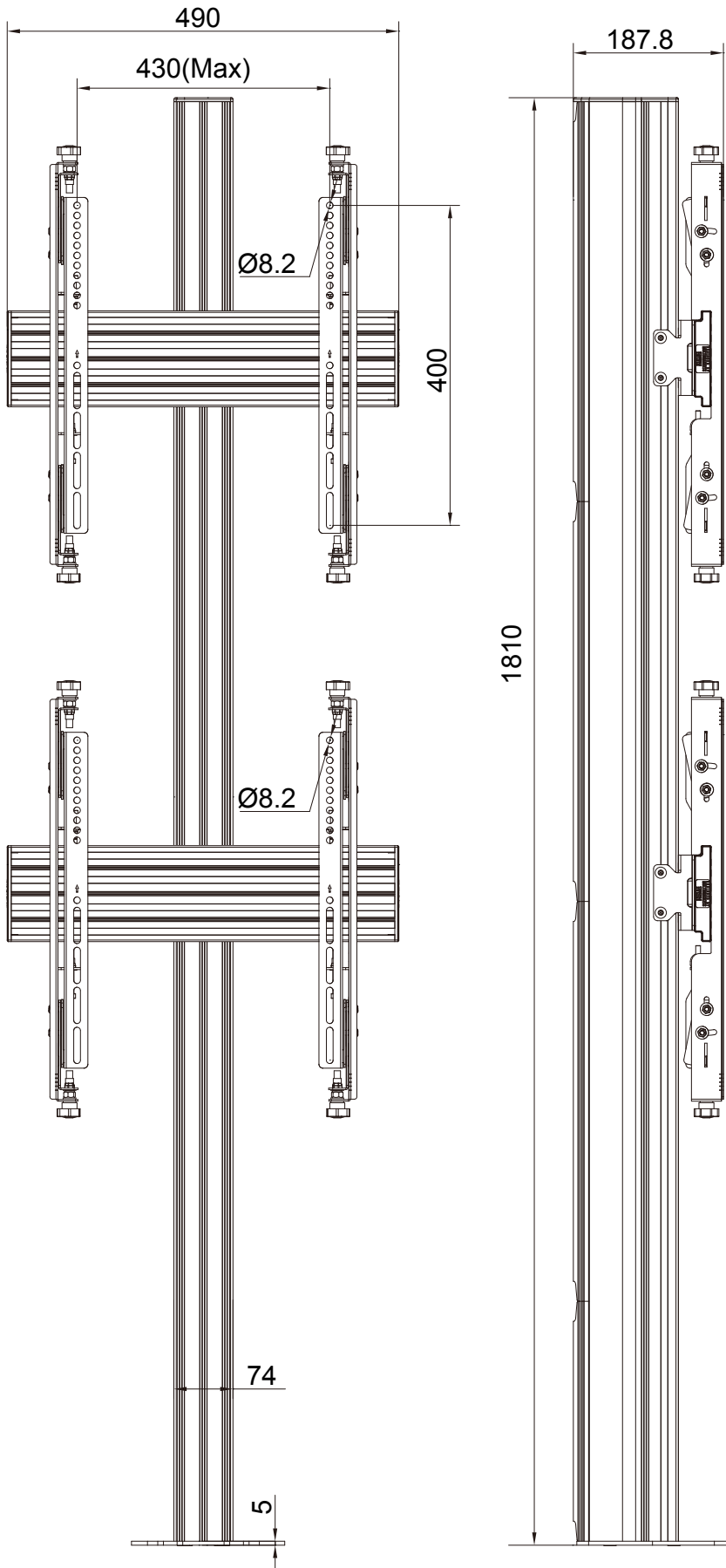
Techniacal measurements(mm)
