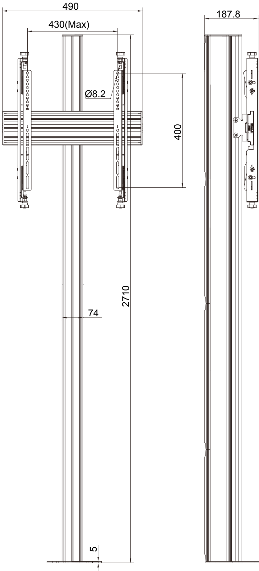
Techniacal measurements(mm)
