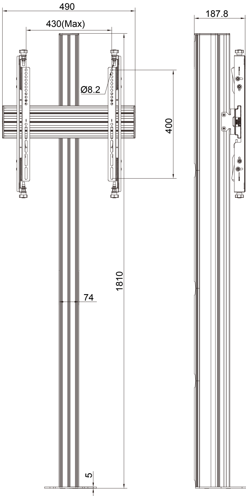
Techniacal measurements(mm)
