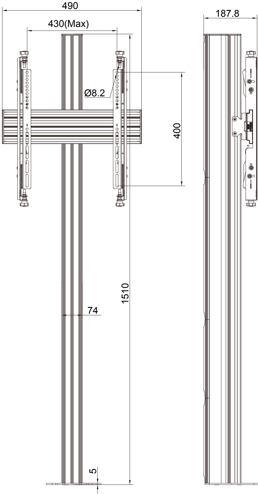
Techniacal measurements(mm)
