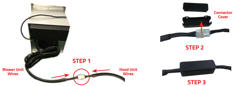
How to connect the blower wires to the hood wires
