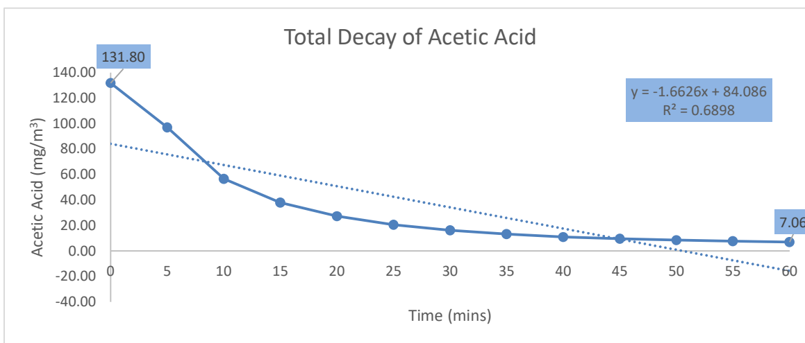
Figure a. Total Decay of VOC (Acetic Acid)
