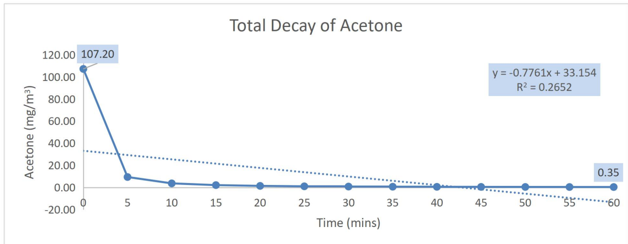
Figure b. Total Decay of Acetone
