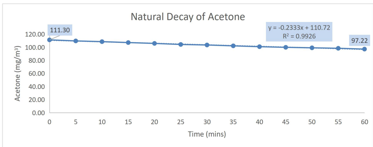
Figure a. Natural Decay of Acetone
