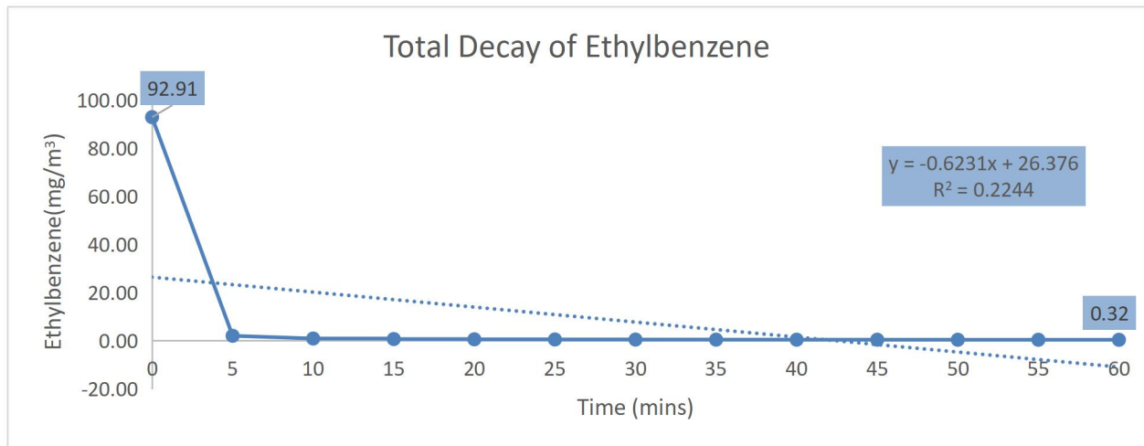
Figure b. Total Decay of Ethylbenzene
