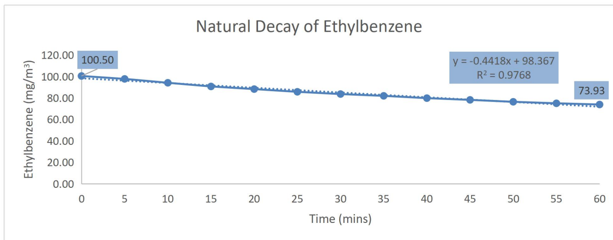
Figure a. Natural Decay of Ethylbenzene
