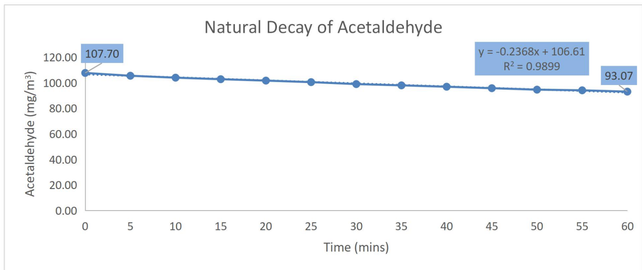
Figure a. Natural Decay of Acetaldehyde
