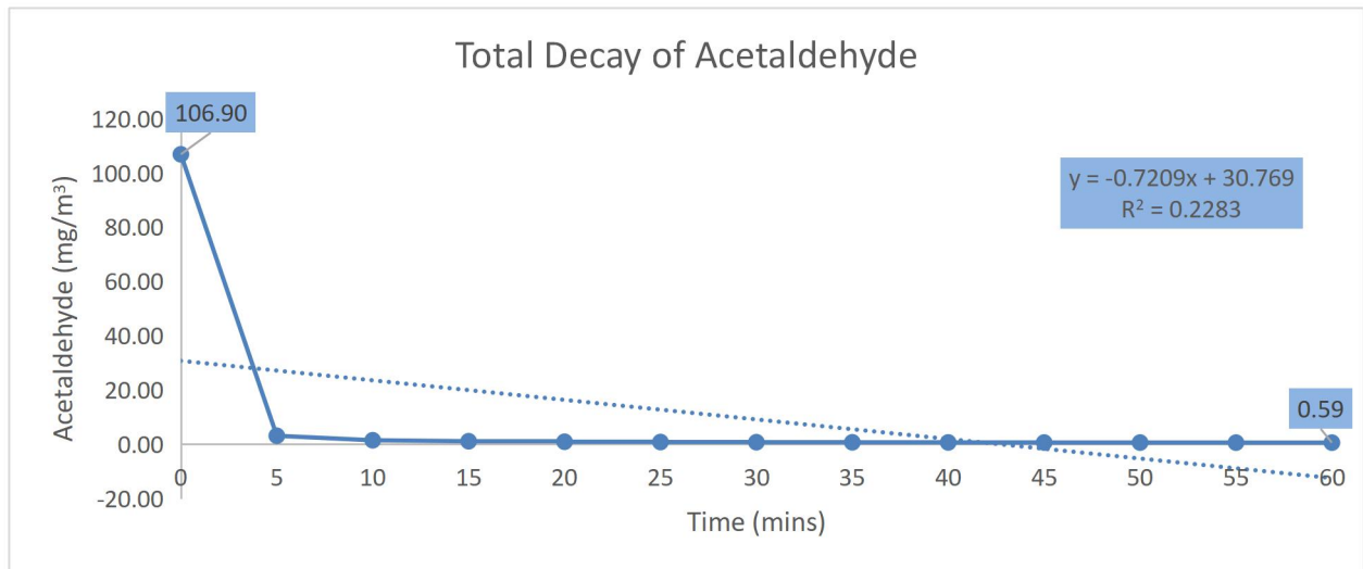
Figure b. Total Decay of Acetaldehyde
