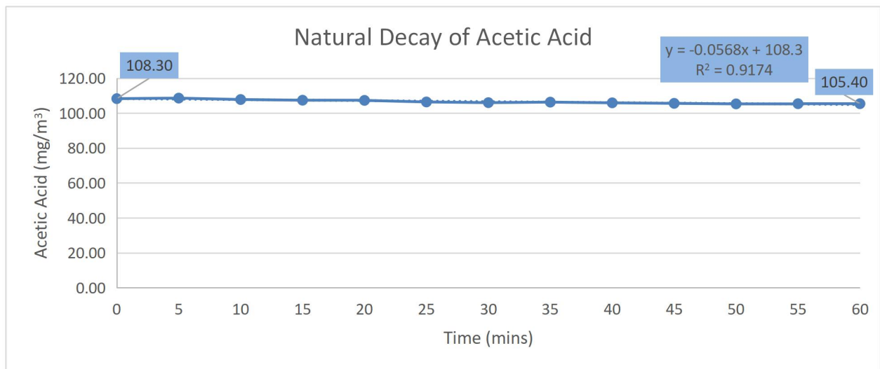
Figure a. Natural Decay of Acetic Acid
