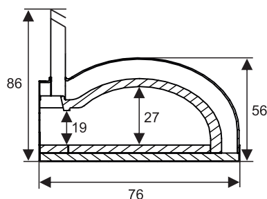
Cross Section
