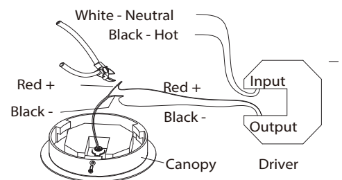
FIG. 3 Driver Wires
