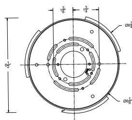
Back Plate Dimensions
