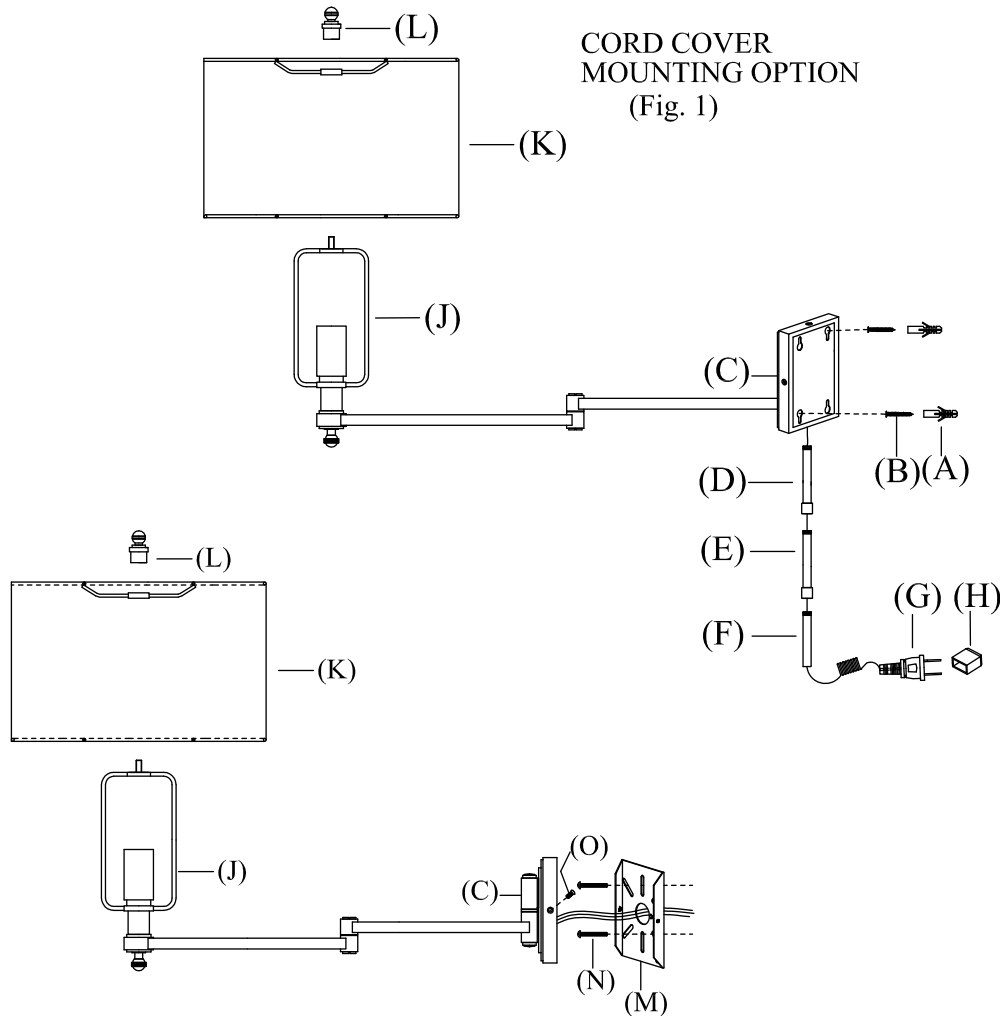
DIRECT WIRE MOUNTING PLATE (Fig. 2)
