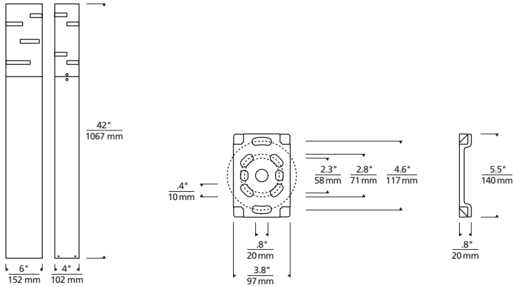
Revel Bollard
