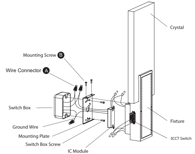
Fig. 2 Mount On Junction Box
