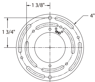
Mounting Ring Dimensions
