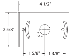
Mounting Back Plate
