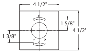
Adapter Plate Dimensions
