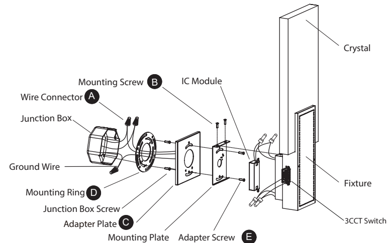
Fig. 2 Mount On Junction Box
