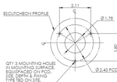
MOUNTING HOLE DETAILS (DIMENSIONS IN INCHES)
