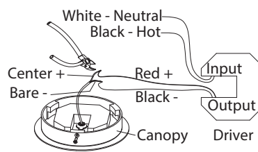
Fig.3 Driver Wiring
