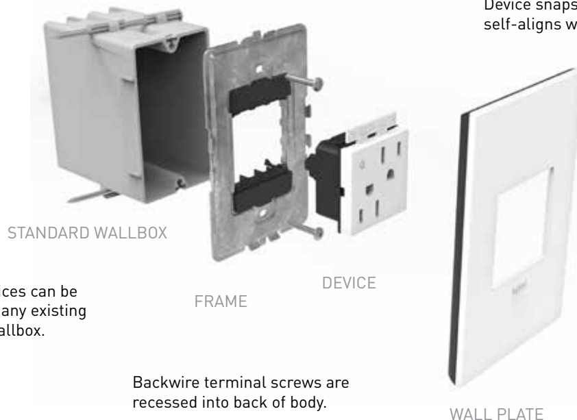
WALL PLATE
