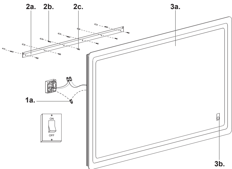
HORIZONTAL MOUNTING
