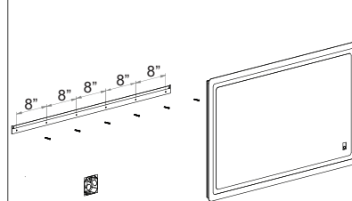
HORIZONTAL MOUNTING
