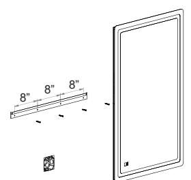
VERTICAL MOUNTING
