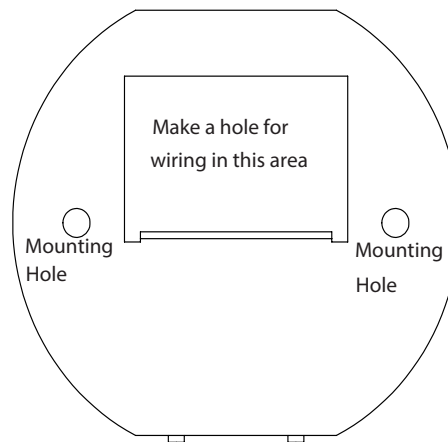
Round mounting diagram
