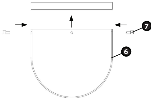
Drawing 2 – GLASS INSTALL
