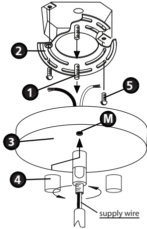
Drawing 1 – Mounting Detail
