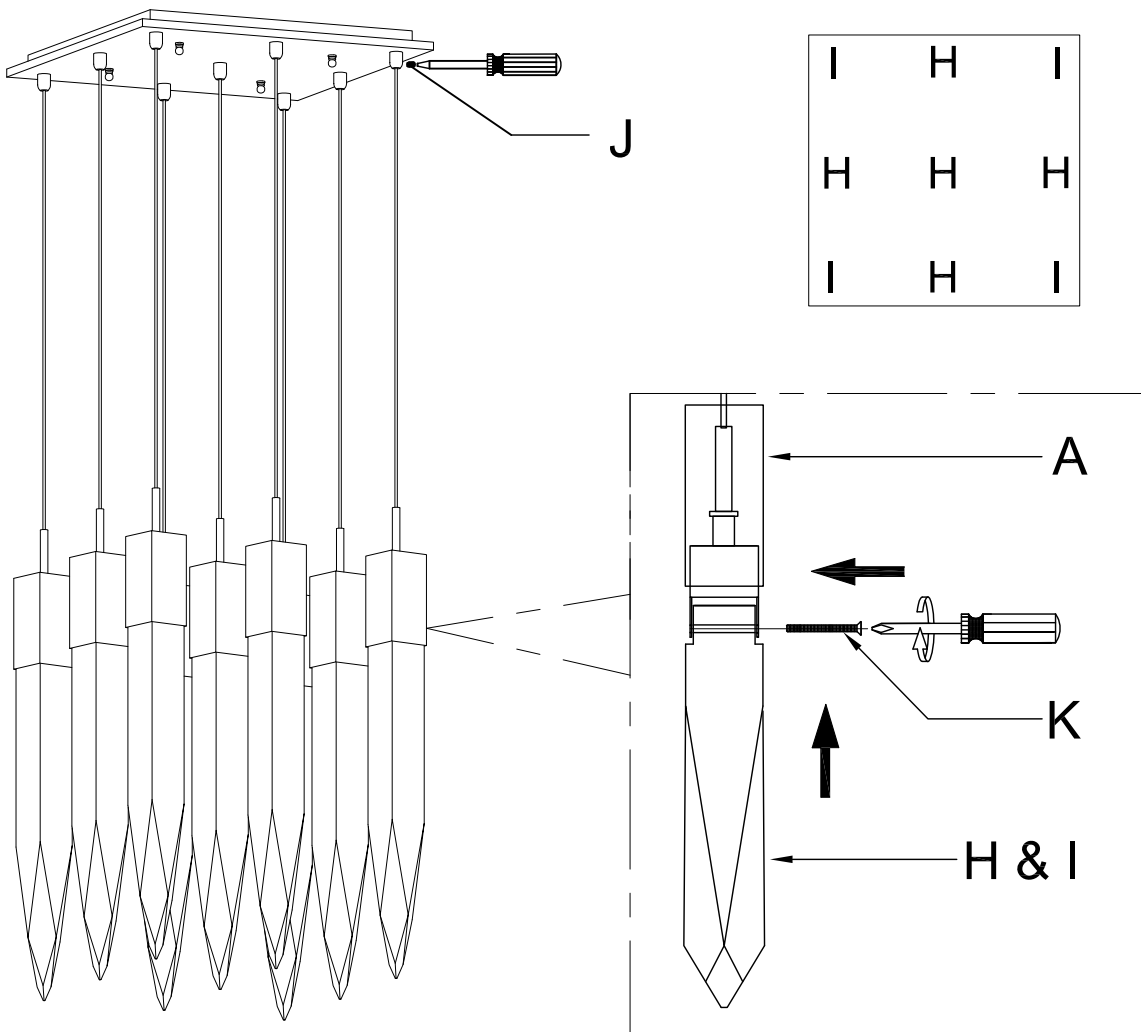
Schematic diagram of glass installation position
