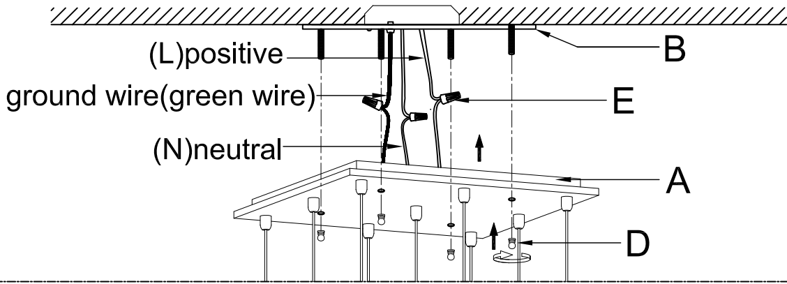
Schematic diagram of glass installation position
