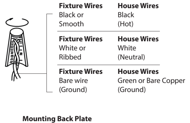
Fig.2 Wiring
