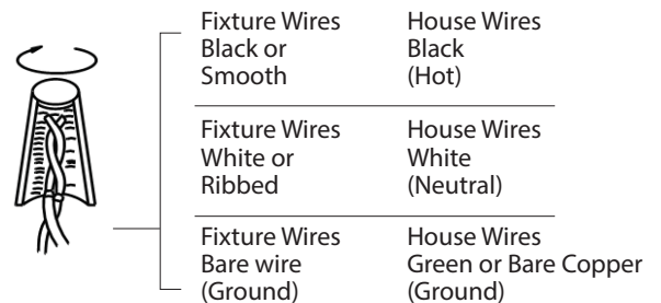
Fig.2 Wiring
