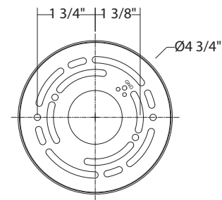
Mounting Back Plate
