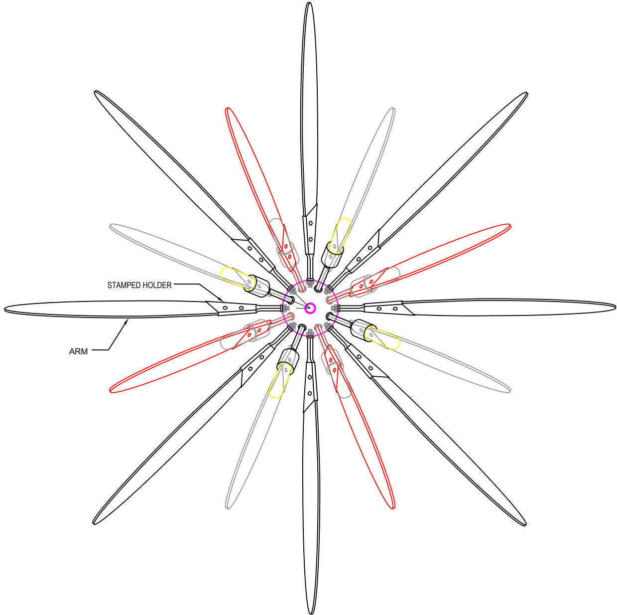
ARM AND STAMPED HOLDER SCHEDULE
