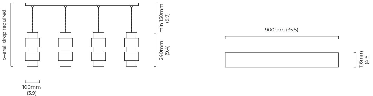
mounting plate dimensions
